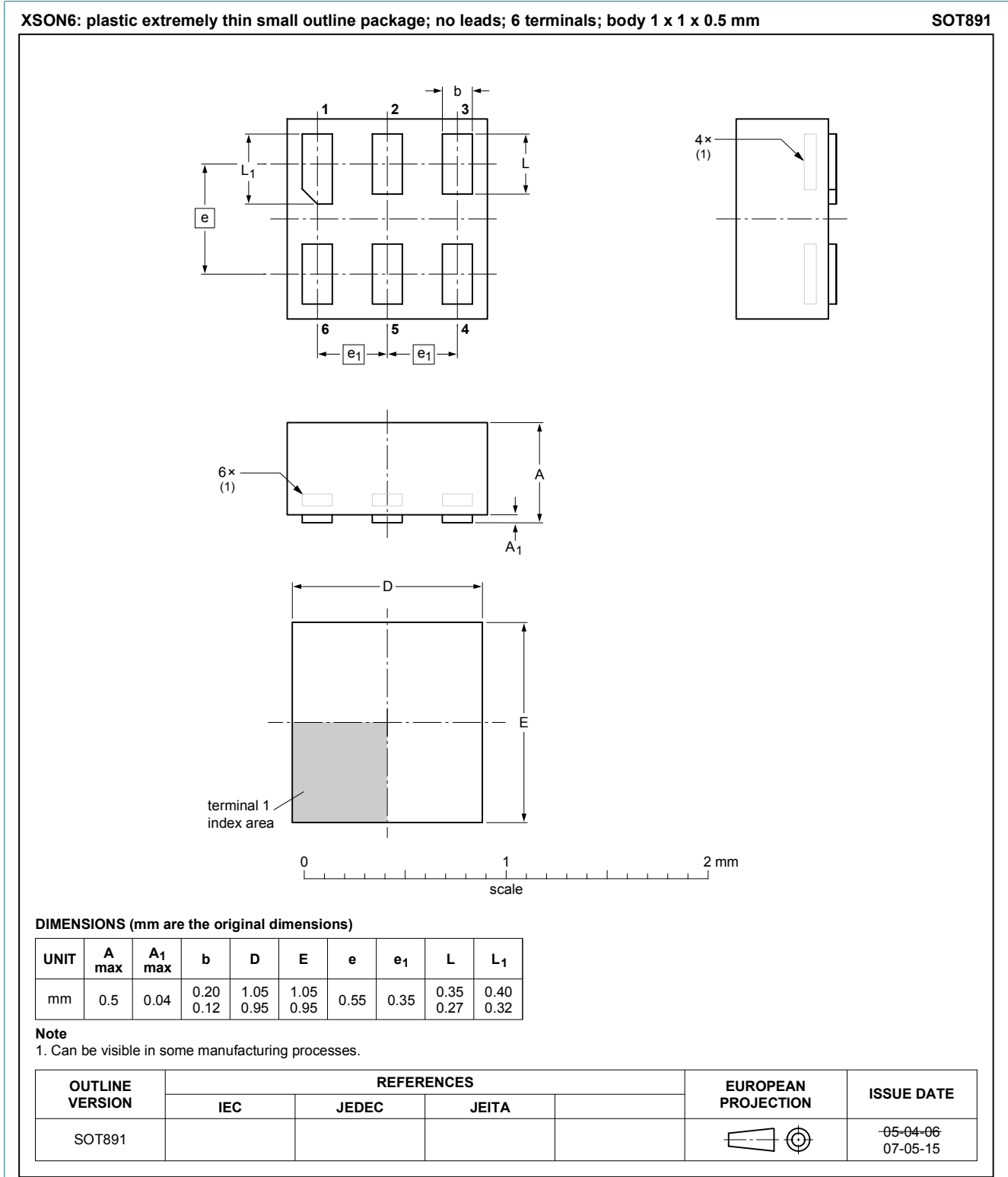
Fig. 1. Package outline XSON6 (SOT891)
